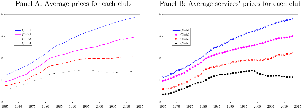
Figure 1: Estimated Common Stochastic Trends for Each Convergent Club
